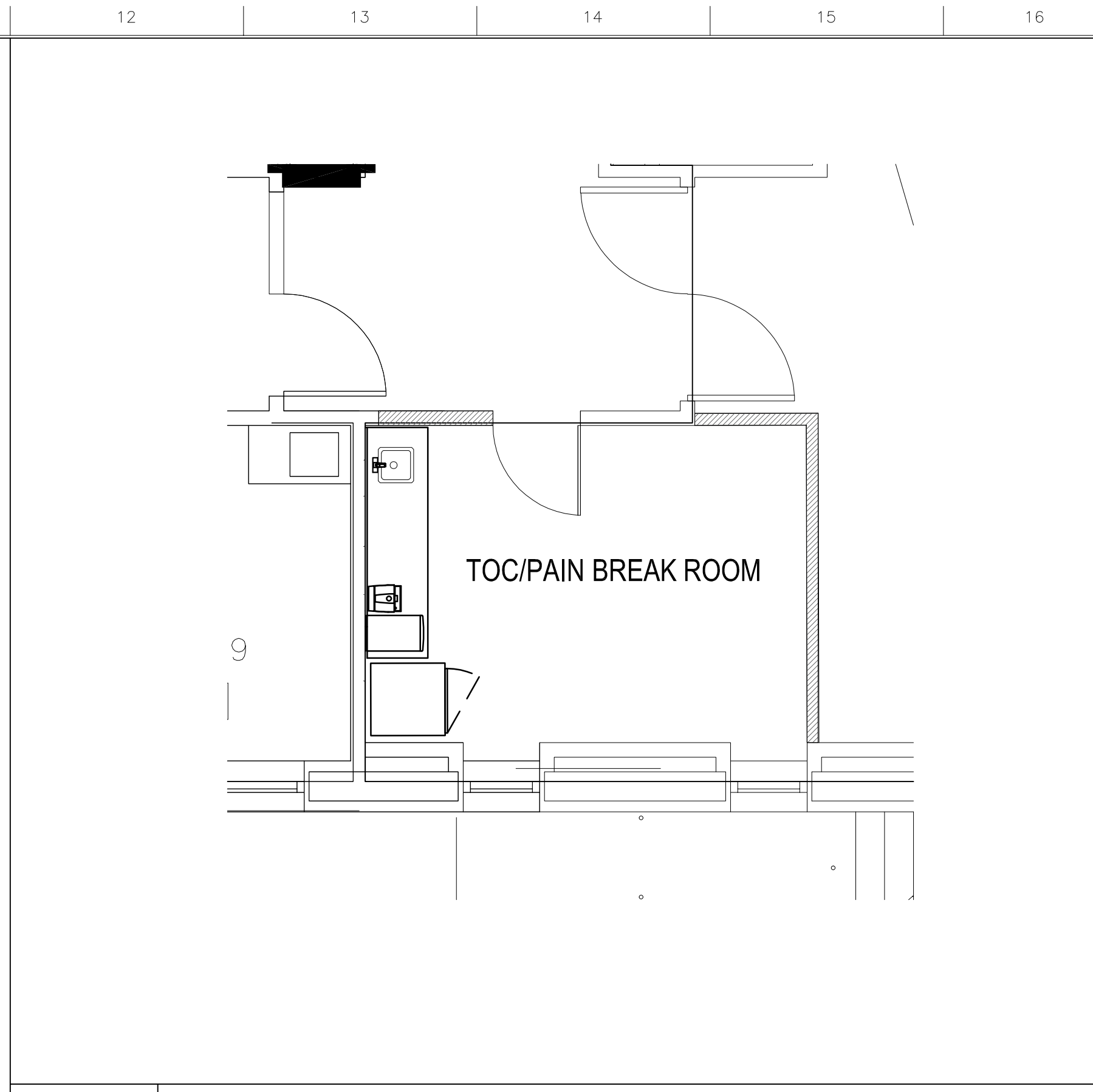
H 12 ENLARGED PLAN - J-WING STAFF LOUNGE 1/2" = 1'-0" A 112
